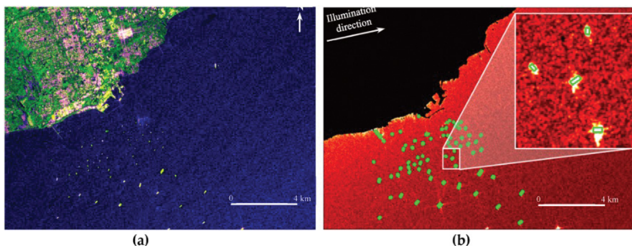
Automatic vessel detection: (a) vessels at the entrance to Port Tema, Ghana (example Sentinel-1 pseudo-colour scene); (b) automatic vessel detection; (b), inset—estimated vessels dimensions and orientation, https://www.mdpi.com/2072-4292/11/3/293/htm
