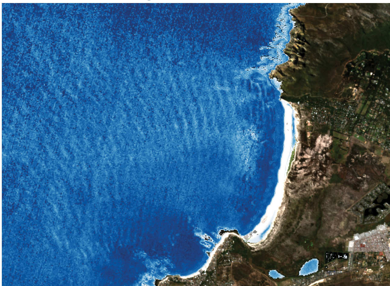
Cape Town, South Africa, Sentinel-2 GeoMAD 2020, MNDWI, processed by Digital Earth Africa
