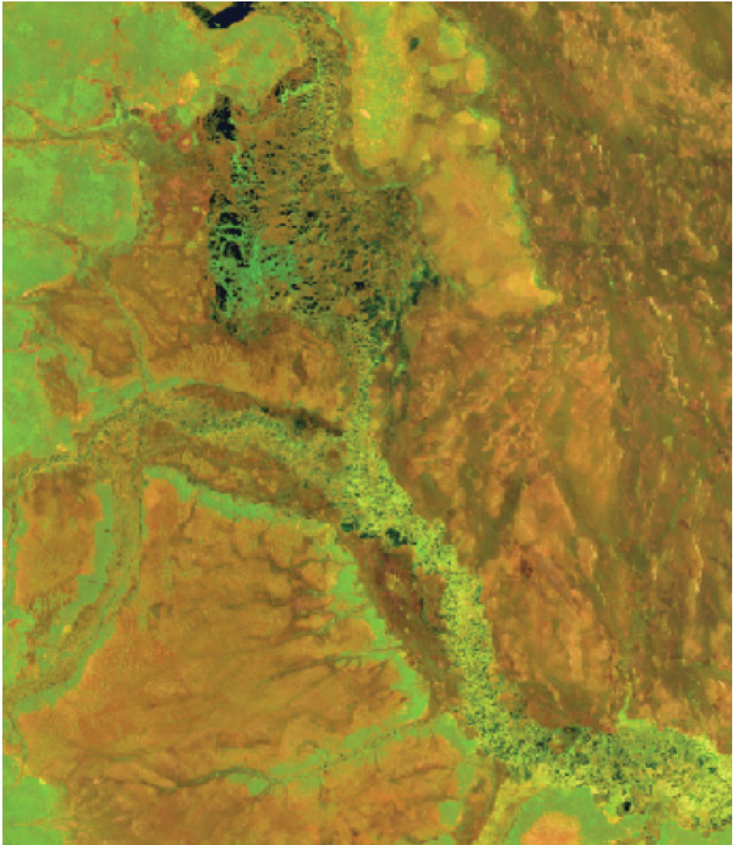
Okavango National Park, Botswana, Sentinel-2 GeoMAD 2021, False Colour, processed by Digital Earth Africa
